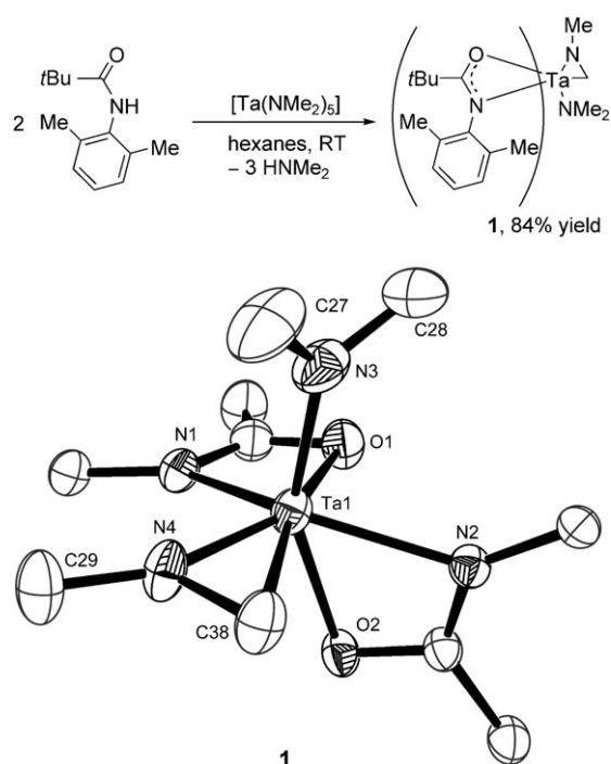
Scheme 2. Synthesis and ORTEP diagram of solid state molecular structure of 1 . Thermal ellipsoids depicted at 50% probability. All hydrogen atoms and most amidate ligand atoms omitted for clarity. Selected bond lengths [Å] and angles [°]: Ta1–N4 1.921(4), Ta1–N3 1.970(5), Ta1–C38 2.178(5), N4–C29 1.451(7), N4–C38 1.424(6), N3–C28 1.459(9), N3–C27 1.463(9), Ta1–N1 2.179(4), Ta1–N2 2.245(4), Ta1–O1 2.214(4), Ta1–O2 2.132(3); N4–Ta1–C38 40.04(17), Ta1–N4–C38 79.7(3), Ta1–N4–C29 155.8(4), Ta1–N3–C27 124.1(5), Ta1–N3–C28 123.0(4), N1–Ta1–O1 59.35(14), N2–Ta1–O2 59.34(12).
